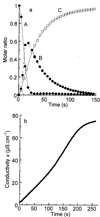
Figure 9. (a) Kinetics of the reaction of \text{CH}_2=\text{CHCH}_2\text{OAc} (10 mM) with the \text{Pd}^0 complex formed from \text{Pd}^0(\text{dba})_2 (2 mM) and dppb (2 mM) in DMF at 25 °C: A (filled diamonds): molar ratio of \text{Pd}^0(\text{dba})(\text{dppb}) versus time, determined by UV spectroscopy at 425 nm; B (filled circles): molar ratio of the neutral intermediate complex (\eta^2\text{-CH}_2=\text{CHCH}_2\text{OAc})\text{Pd}^0(\text{dppb}) versus time, determined from curves A and C [ B = 1 - (A + C) ]; C (empty squares): molar ratio of the cationic complex [(\eta^3\text{-CH}_2\text{CHCH}_2)\text{Pd(dppb)}]^+\text{AcO}^- versus time, determined by conductivity measurements; (b) kinetics of the reaction of \text{CH}_2=\text{CHCH}_2\text{OAc} (10 mM) with the \text{Pd}^0 complex formed from \text{Pd}^0(\text{dba})_2 (2 mM) and dppf (2 mM) in DMF at 16 °C, monitored by conductivity measurements of the cationic complex [(\eta^3\text{-CH}_2\text{CHCH}_2)\text{Pd(dppf)}]^+\text{AcO}^-
