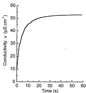
Figure 3. Kinetics of the formation of [\text{CH}_2=\text{C}(\text{nBu})\text{Pd}(\text{PPh}_3)_2(\text{DMF})]^+\text{TfO}^- in the oxidative addition of \text{CH}_2=\text{C}(\text{nBu})\text{OTf} (2 mM) to [\text{Pd}^0(\text{PPh}_3)_4] (2 mM) in DMF at 10 °C; variation of the conductivity \kappa versus time; \kappa = \kappa_{\text{exp}} - \kappa_0 ( \kappa_{\text{exp}} : experimental conductivity at t ; \kappa_0 : initial residual conductivity of 3 \mu\text{S}\cdot\text{cm}^{-1} )
