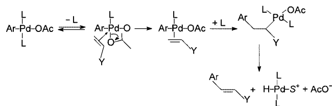
Scheme 11. Mechanism of the carbopalladation step from \text{ArPd(OAc)(PPh}_3)_2 complexes followed by \beta -hydride elimination in DMF
