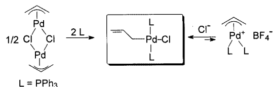
Scheme 19. Formation of (\eta^1\text{-allyl})(\text{chloro})\text{palladium} complexes
