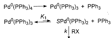
Scheme 3. Mechanism of oxidative additions from \text{Pd}^0(\text{PPh}_3)_4 ( \text{S} = \text{solvent} )
