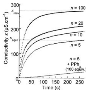
Figure 4. Conductivity in DMF of [\text{HPd}(\text{PPh}_3)_2(\text{DMF})]^+\text{AcO}^- generated in the reaction of \text{Pd}^0(\text{PPh}_3)_4 (2 mM) with n equiv. of acetic acid: n = 100, 20, 10 , and 5 in the absence of \text{PPh}_3 , or n = 5 in the presence of 100 equiv. of \text{PPh}_3 (as indicated in the Figure) at 25 °C
