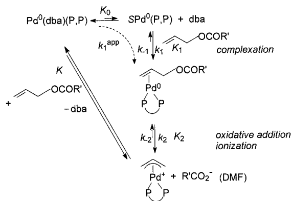
Scheme 16. Mechanism of the reversible reaction in DMF of allyl carboxylates with the \text{Pd}^0 complex formed from \text{Pd}^0(\text{dba})_2 and 1 equiv. of (P,P) ligand (dppb, dppf)
