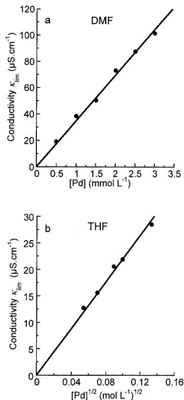
Figure 2. (a) Variation of the conductivity of trans - [\text{4-O}_2\text{NC}_6\text{H}_4\text{Pd(PPh}_3)_2(\text{DMF})]^+\text{TfO}^- in DMF, determined by the value of \kappa_{\text{lim}} (Figure 1, a) versus the concentration of Pd initially introduced as \text{Pd}^0(\text{PPh}_3)_4 before reaction with 4\text{-O}_2\text{NC}_6\text{H}_4\text{OTf} , at 20 °C; (b) variation of the conductivity of trans - [\text{4-O}_2\text{NC}_6\text{H}_4\text{Pd(PPh}_3)_2(\text{THF})]^+\text{TfO}^- in THF (determined as in Figure 2, a) versus the square root of the Pd concentration, at 20 °C
