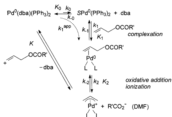
Scheme 14. Mechanism of the reversible reaction of allyl carboxylates with the \text{Pd}^0 complexes generated from \text{Pd}^0(\text{dba})_2 and \text{PPh}_3 (2 equiv.) in DMF
